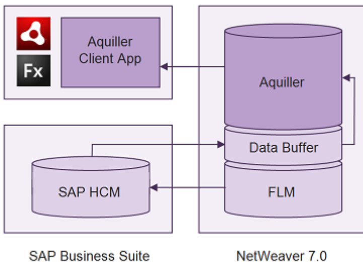
Figure 1: Aquiller Architecture
